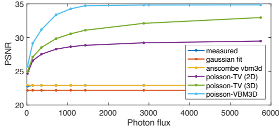
Figure 8. Evaluation of PSNR for the simulated results in Figure 7. The photon flux corresponds to the intensity of the light source used to generate the simulated measured image.
