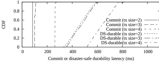
Figure 20: Latency of slow commit and replication.
